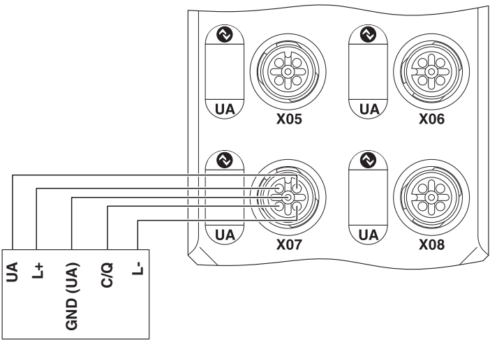
Connection diagram
